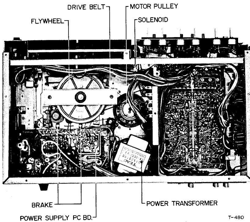
Fig. 5-3 Bottom View
