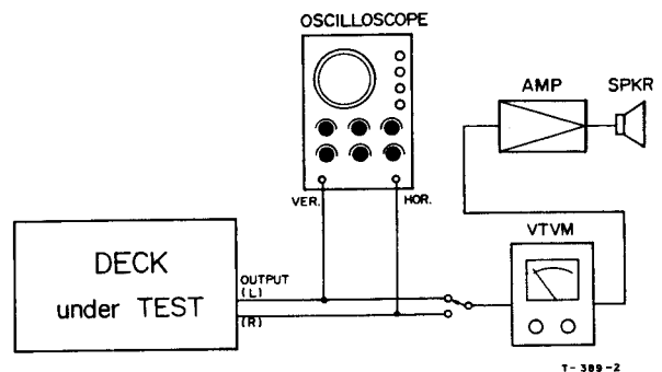
Fig. 7-3 Connection
