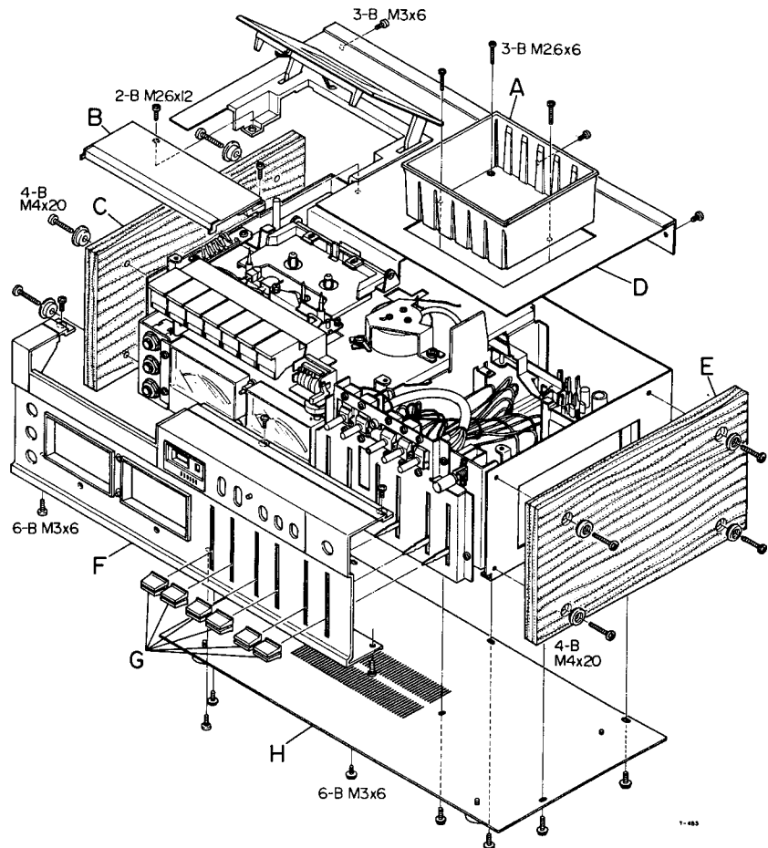
Fig. 3-1 Case/Front Panel Removal
