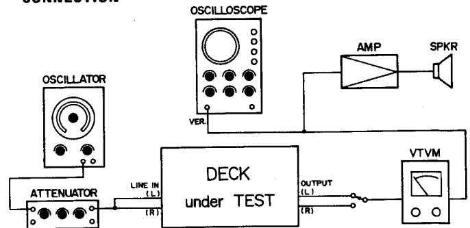
Fig. 7-10 Connection
