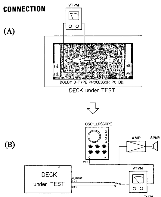
Fig. 7-4 Connections
