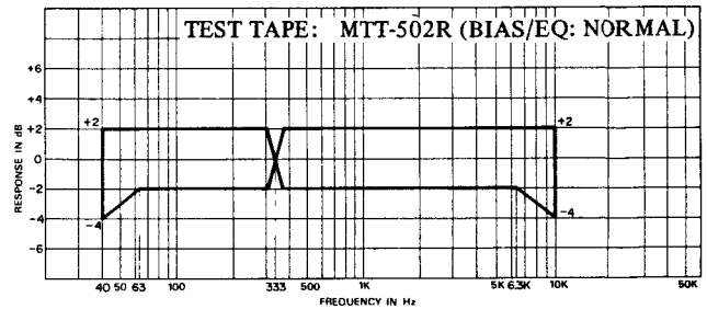
Fig. 10-3 Overall Frequency Response Limits (for BIAS/EQ: NORMAL)
