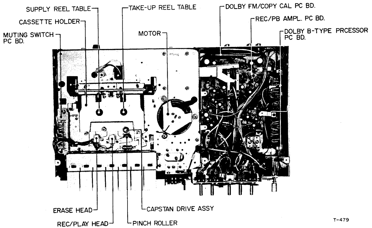
Fig. 5-2 Top View
