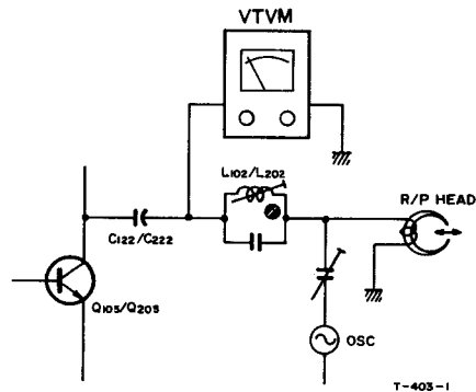
Fig. 7-11 Connection
