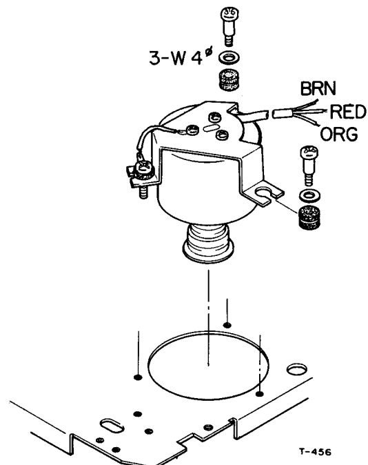
Fig. 3-2 Motor Replacement
